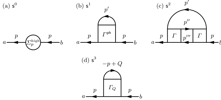
Fig. 1: Self-energy diagrams and their order of magnitude in the small expansion parameter, s \in \{k_B T_c / E_f, 1 / k_f \xi\} of Fermi liquid theory. (a) \Sigma_p^{\text{high}} is \mathcal{O}(s^0) and gives quasiparticle the mass renormalization, (b) is the Landau mean field self-energy of \mathcal{O}(s^1) , (c) is the self-energy from binary collision scattering and is \mathcal{O}(s^2) , and (d) is the self-energy for quasiparticles-pair fluctuation interactions, is \mathcal{O}(s^3) ; vertex \Gamma_Q diverges for T \rightarrow T_c^+ and Q \rightarrow 0 .
