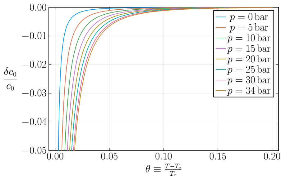
Fig. 2: The deviation of the zero sound velocity relative to its Fermi liquid value, \delta c_0/c_0 , at different pressures. The curves are calculated with a fixed cut-off x_c = 0.236 .
