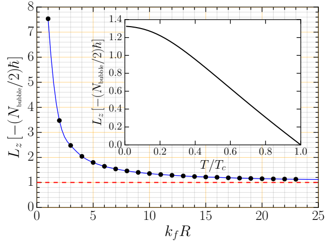
FIG. 7. (Color online) Angular momentum of hard sphere “bubbles” embedded in {}^3\text{He-A} as a function of hard sphere radius, k_f R . For an electron bubble, k_f R = 11.17 . In the macroscopic limit, R \gg \xi_0 (red dashed line), L_z scales to L_z^\infty = -(N_{\text{bubble}}/2)\hbar . Inset: Temperature dependence of L_z for the electron bubble.
