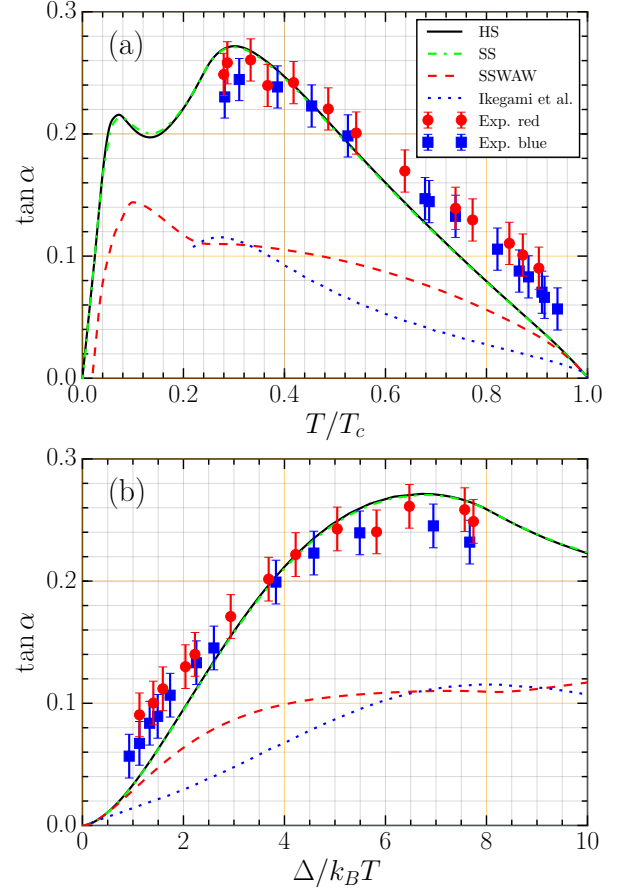
FIG. 12. (Color online) Panel (a): Hall ratio for the motion of electron bubbles in {}^3\text{He-A} , \tan \alpha \equiv v_y/v_x = \eta_{xy}/\eta_{xx} , as a function of temperature for the hard sphere model for the quasiparticle-ion potential with k_f R = 11.17 (black line). The experimental data was from the RIKEN group. 8,9 Theoretical results for the repulsive soft core potential (dashed green line) and repulsive potential with short-range attraction (dashed red line) are shown for comparison. The dotted blue line corresponds to the calculation based on the formulas from Salmelin et al. 23,24 presented in Refs [8 and 9]. Panel (b): The same results presented as a function of \Delta(T)/k_B T .
