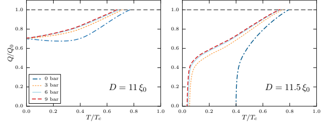
FIG. 6 Temperature and pressure dependence of the wavenumber Q for film thicknesses D = 11\xi_0 , with no Stripe to B transition (left panel), and D = 11.5\xi_0 , with a Stripe to B transition (right panel). The onset of the Stripe transition is based on the Planar-Stripe instability, i.e. omitting the A phase.
