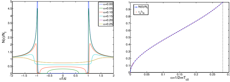
Fig. 4 (Color online) Density of states as a function of excitation energy from weak pair breaking (left). Comparison of the normalized density of states at the Fermi level (right panel), N(0)/N_f obtained by direct calculation from Eq. (24), and the Sommerfeld ratio, \gamma_s/\gamma_N computed from the limit, \lim_{T \rightarrow 0} C_S/T .
