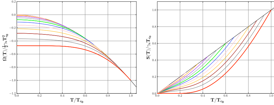
Fig. 2 (Color online) Thermodynamic potential (left panel) and entropy (right panel) for the B-phase of {}^3\text{He} -aerogel in the unitary limit as a function of T/T_{c0} for pair breaking ranging from 0 \leq \alpha \leq 0.275 in steps of 0.025. Results for pure {}^3\text{He-B} are shown as red curves.
