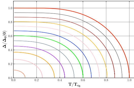
Fig. 1 (Color online) Suppression of the B-phase order parameter in the unitary limit as a function of \alpha = 1/2\pi\tau T_{c_0} . \Delta(T) is normalized by \Delta_0(0) = 1.78k_B T_{c_0} for pure ^3\text{He-B} in the weak-coupling limit (red curve). The curves for 0 < \alpha \leq 0.275 are shown for \alpha in steps of 0.025.
