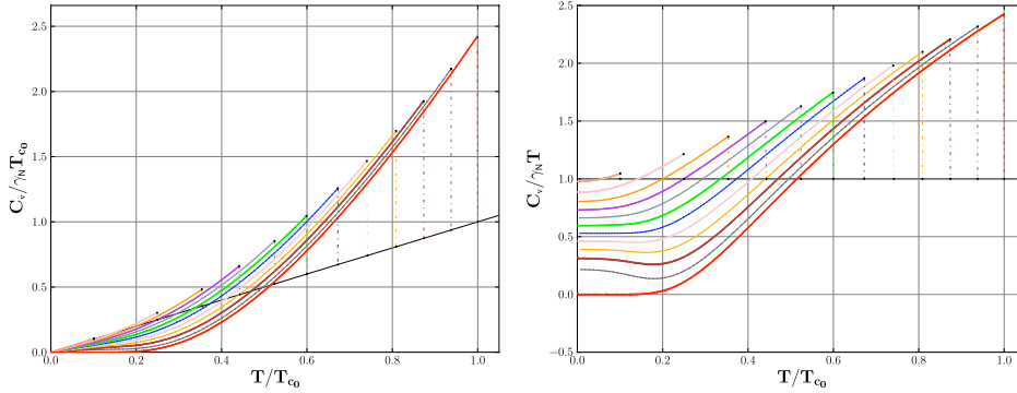
Fig. 3 (Color online) Specific heat capacity normalized by \gamma_N T_{c_0} (left panel) and by \gamma_N T (right panel) for the B-phase of ^3\text{He} -aerogel in the unitary limit as a function of T/T_{c_0} for pair breaking ranging from 0 \leq \alpha \leq 0.275 in steps of 0.025. Results for pure ^3\text{He} -B are shown as red curves.
